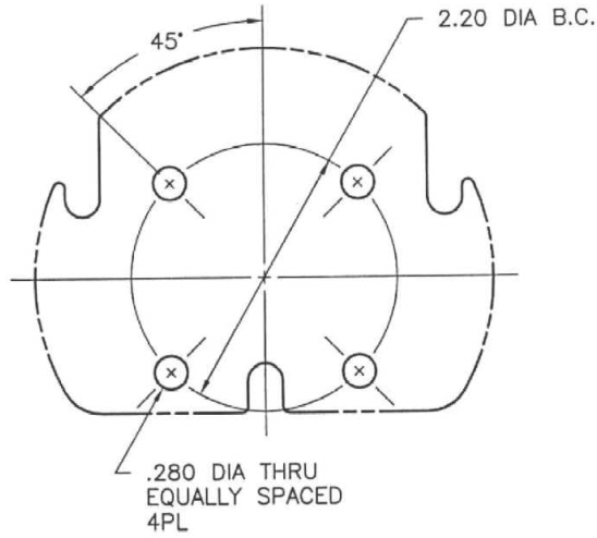
MOUNTING PATTERN OPTION 1
