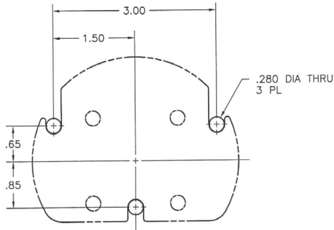
MOUNTING PATTERN OPTION 2
